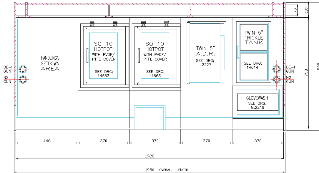
PART SECTION SHOWING DECKTOP LAYOUT.
