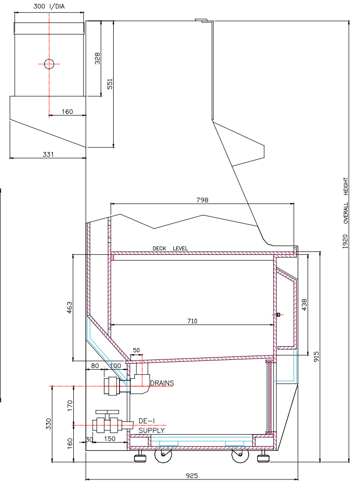
PART SECTIONAL END ELEVATION
